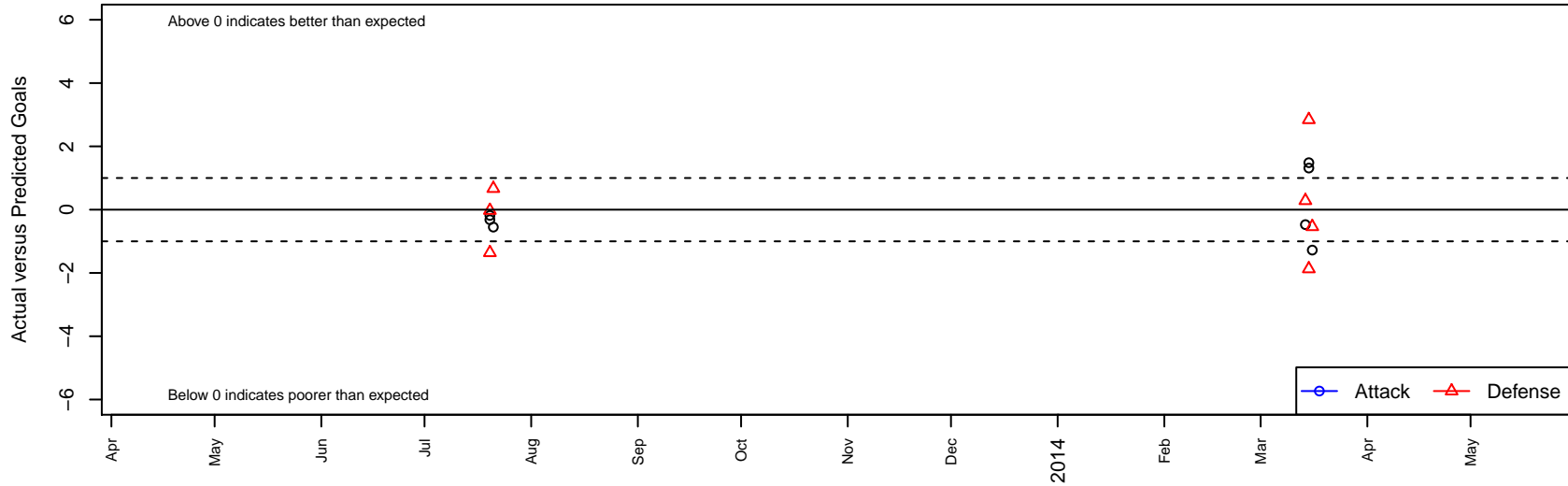
Pateadores IER B96 Dots are actual minus expected GF (blue circles) and GA (red triangles). Blue line is smoothed change in attack strength. Red is smoothed change in defense strength.
